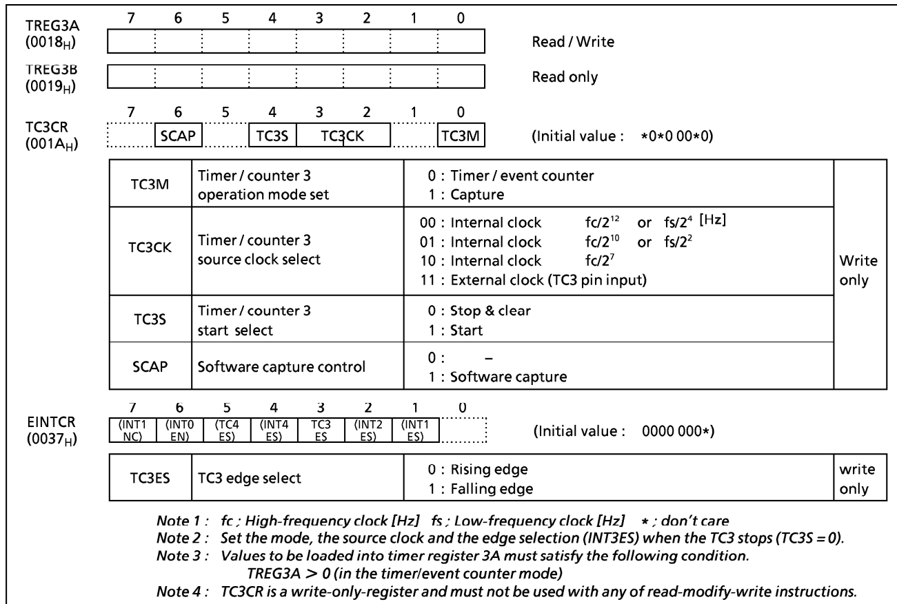
Figure 2-29. Timer Register 3 and TC3 Control Registers
