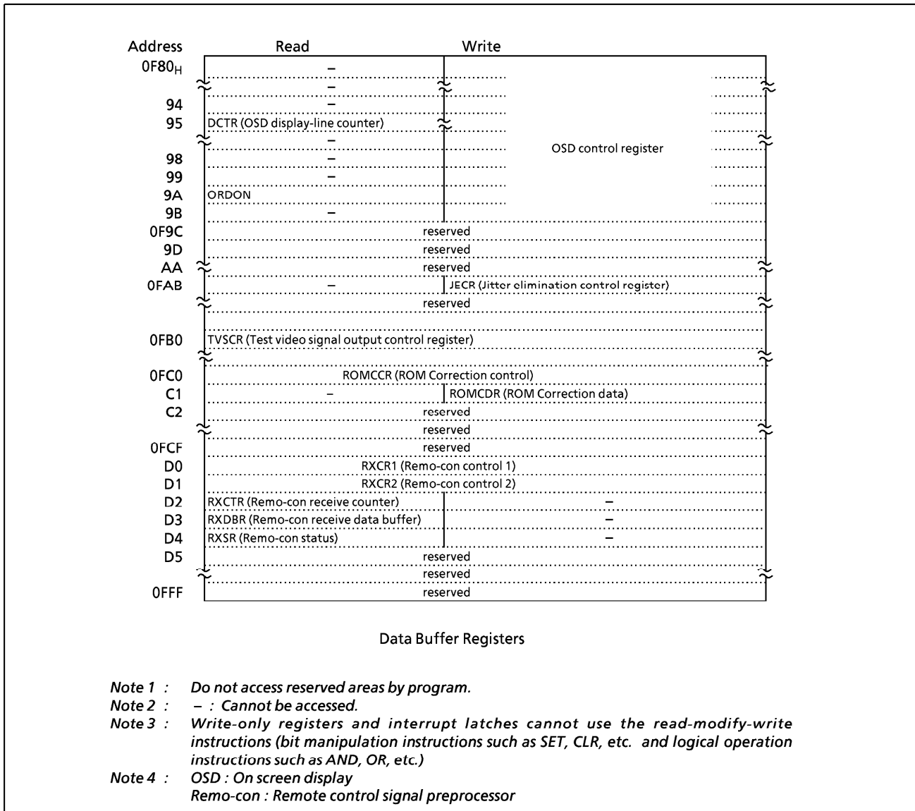
Figure 2-2. DBR
