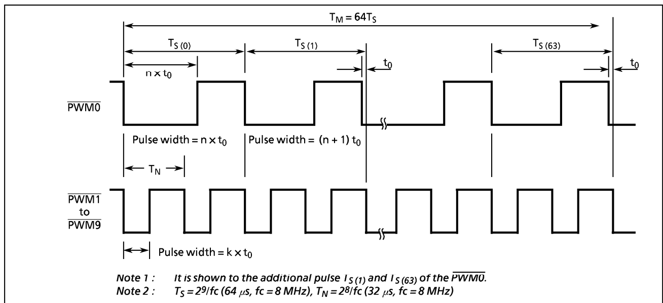
Figure 2-73. PWM Output Wave Form
