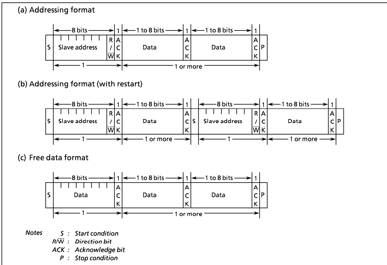
Figure 2-34. Data Format
