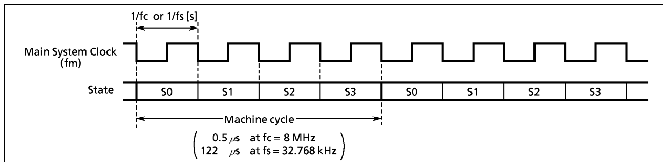
Figure 1-14. Machine Cycle
