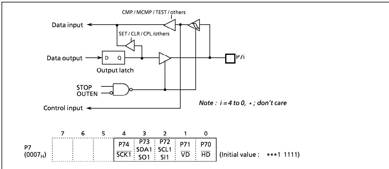
Figure 2-11. Port P7
