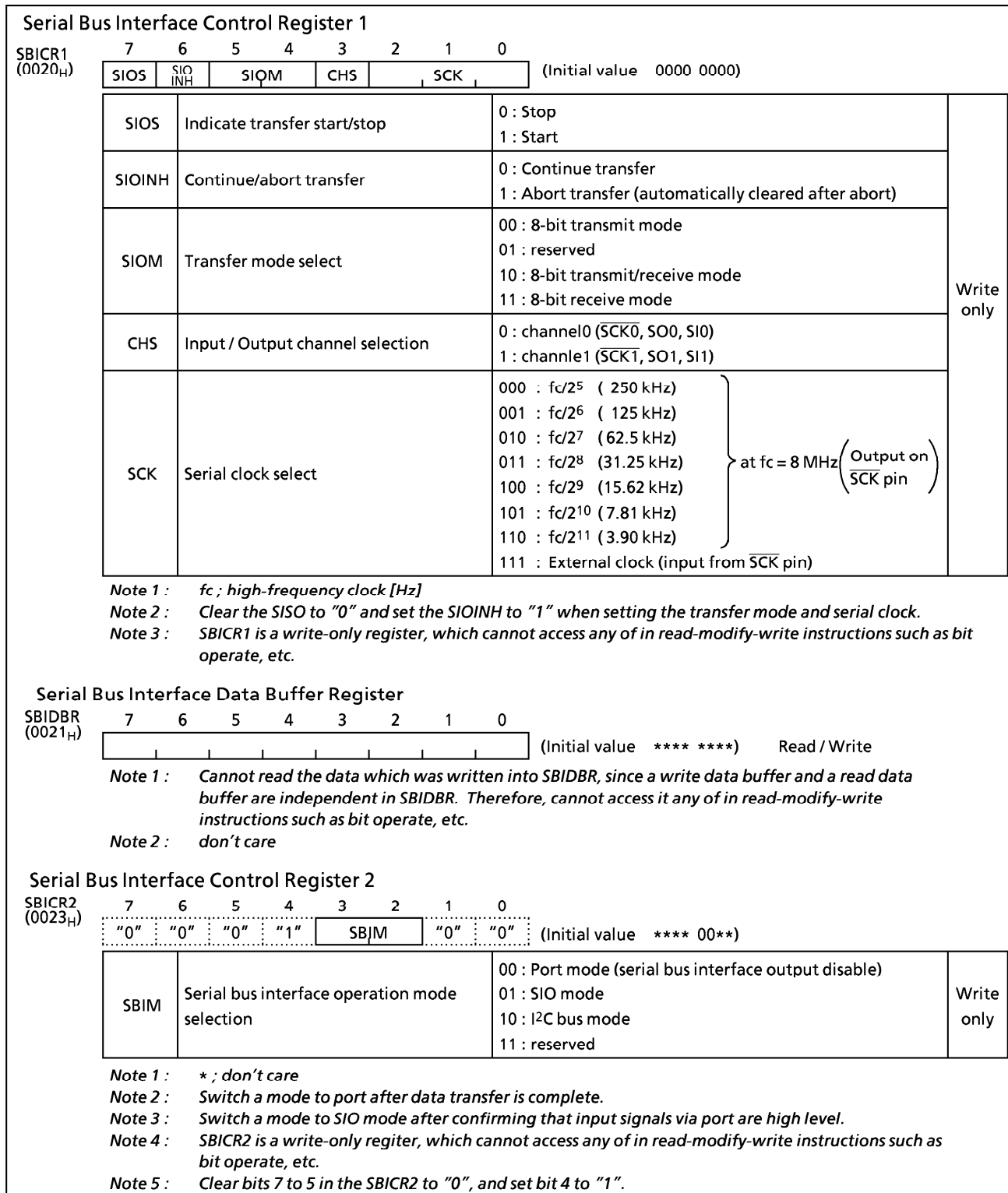
Figure 2-49. Serial Bus Interface Control Register 1 / Serial Bus Interface Data Buffer Register / Serial Bus Interface Control Register 2 in SIO Mode
