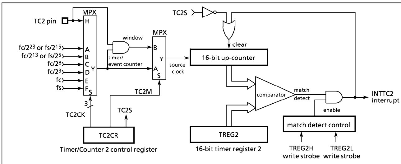
Figure 2-25. Timer / Counter 2 (TC2)
