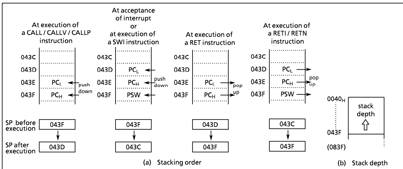
Figure 1-9. Stack
