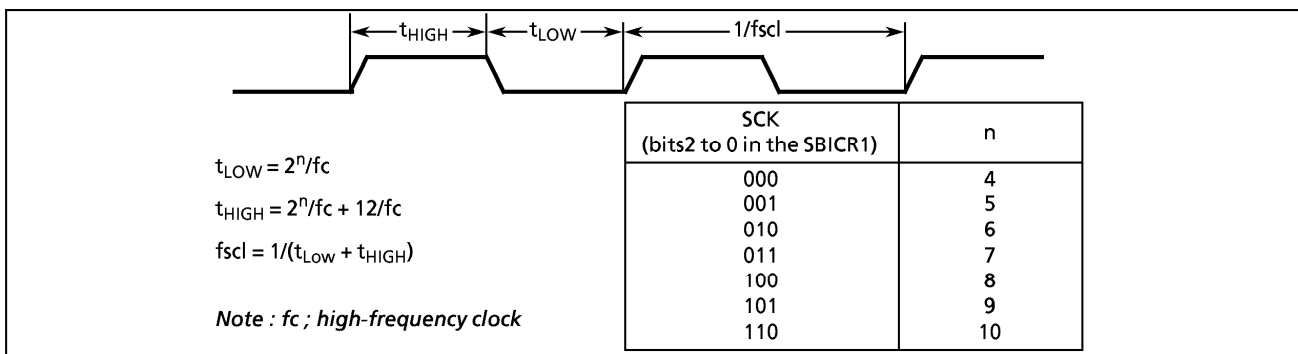
Figure 2-37. Clock Source
