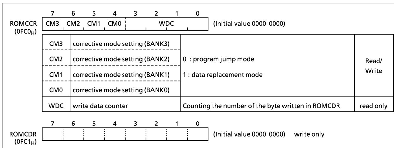
Figure 1-34. ROM Corrective Control Register and ROM Corrective Data Register
