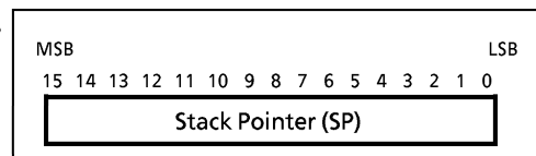
Figure 1-8. Stack Pointer
