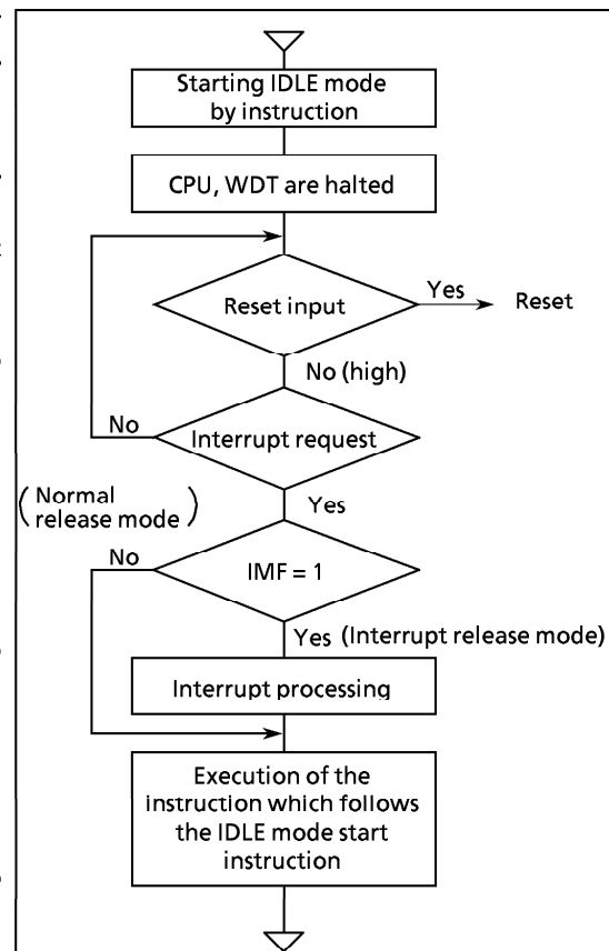
Figure 1-20. IDLE Mode
