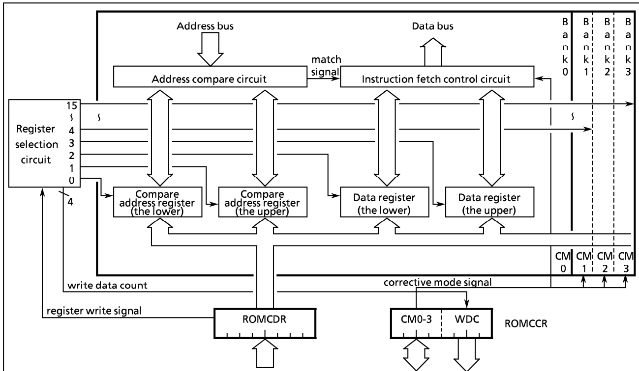
Figure 1-33. ROM Corrective Circuit
