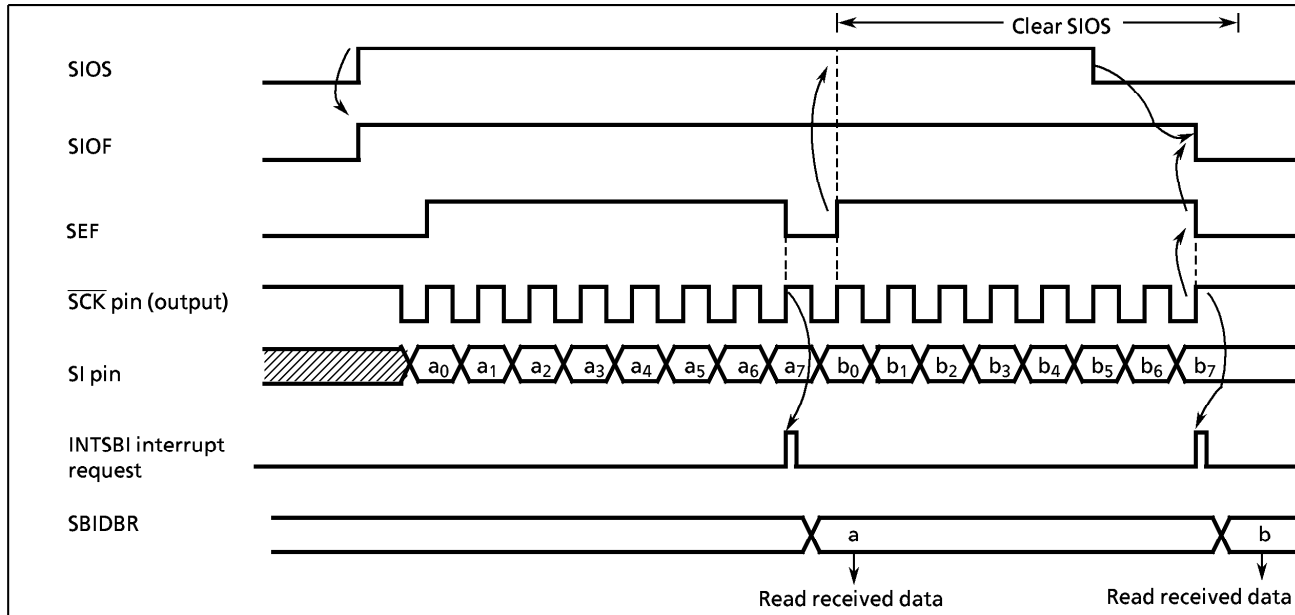
Figure 2-56. Receive Mode (Example : Internal clock)
