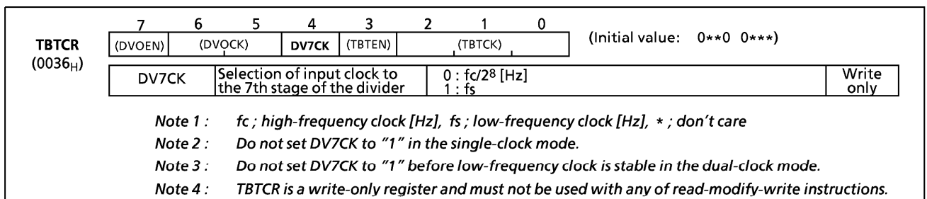
Figure 1-13. Timing Generator Control Register
