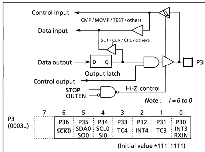
Figure 2-7. Port P3
