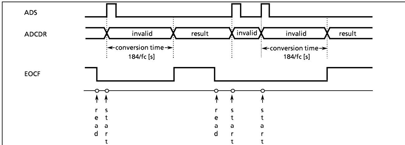
Figure 2-70. A/D Conversion Timing Chart
