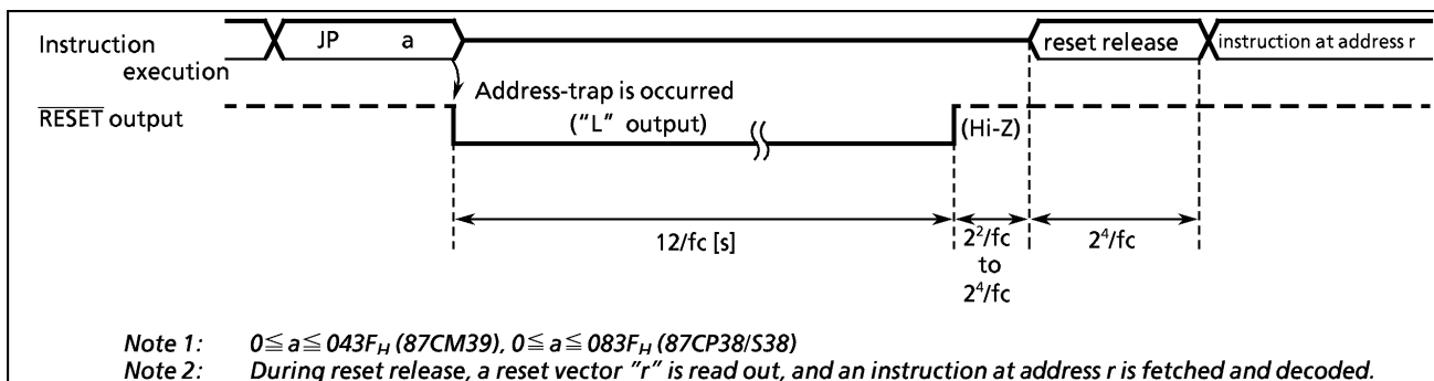
Figure 1-32. Address-Trap-Reset
