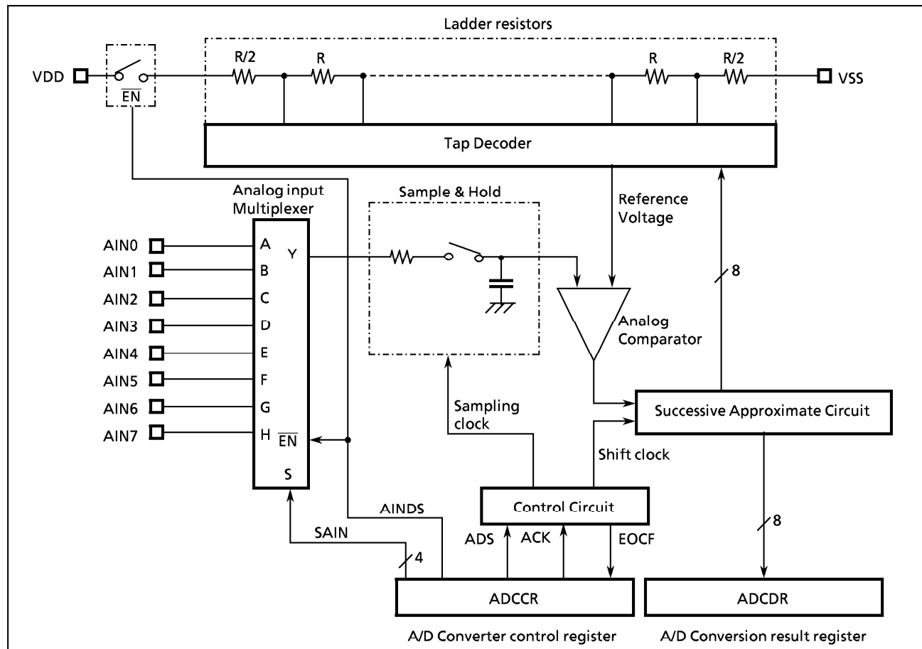
Figure 2-67. A/D Converter
