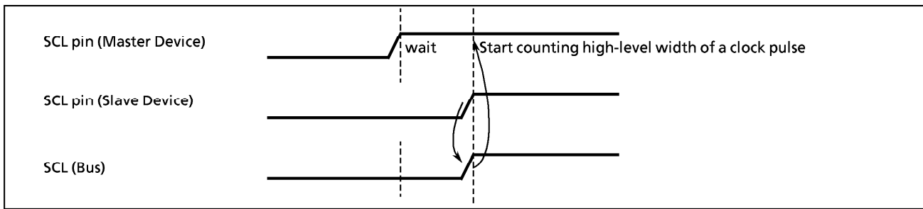
Figure 2-38. Clock Synchronization
