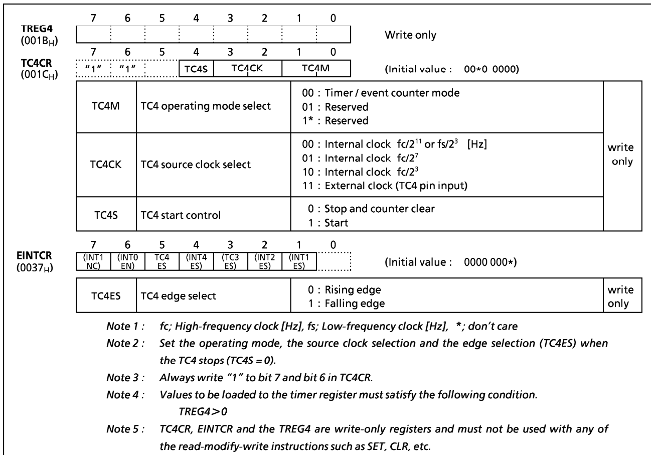
Figure 2-32. Timer Register 4 and TC4 Control Registers
