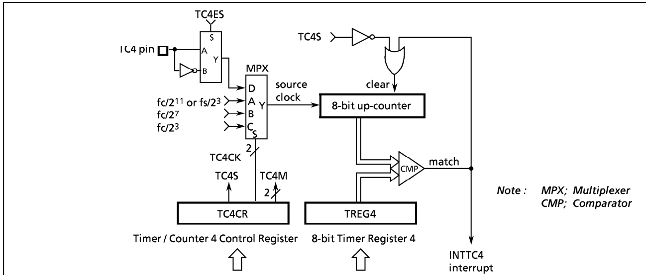
Figure 2-31. Timer / Counter 4
