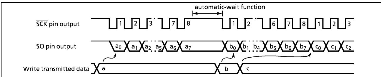
Figure 2-51. Automatic-wait Function
