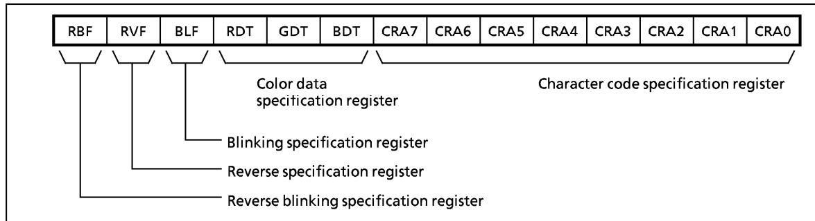
Figure 2-81. Display Memory Bit Configuration
