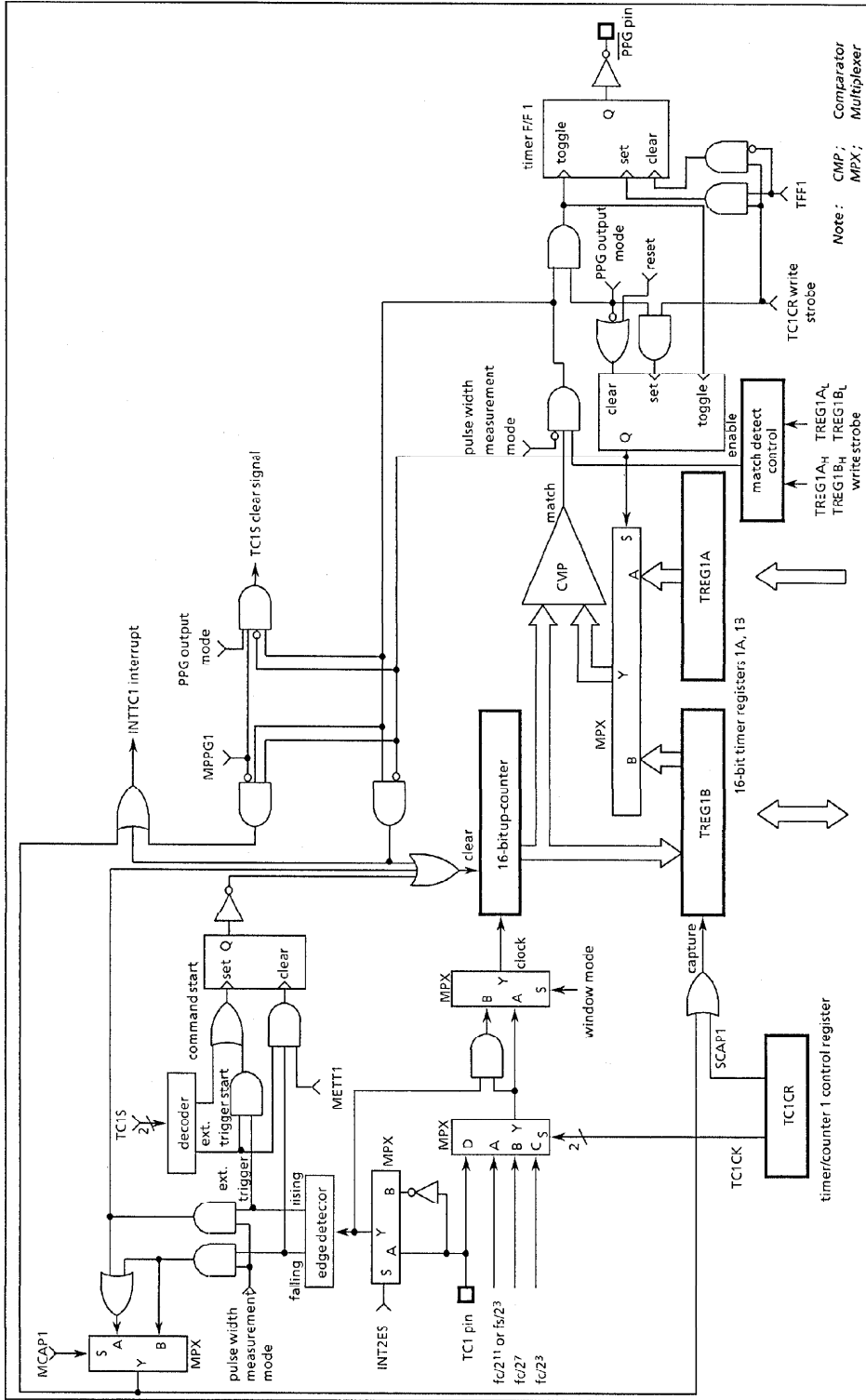
Figure 2-16. Timer / Counter 1
