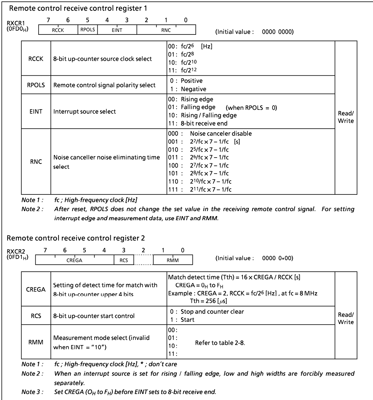
Figure 2-60. Remote Control Receive Control Register 1, 2
